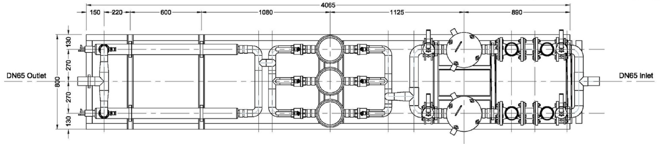
PLAN VIEW
