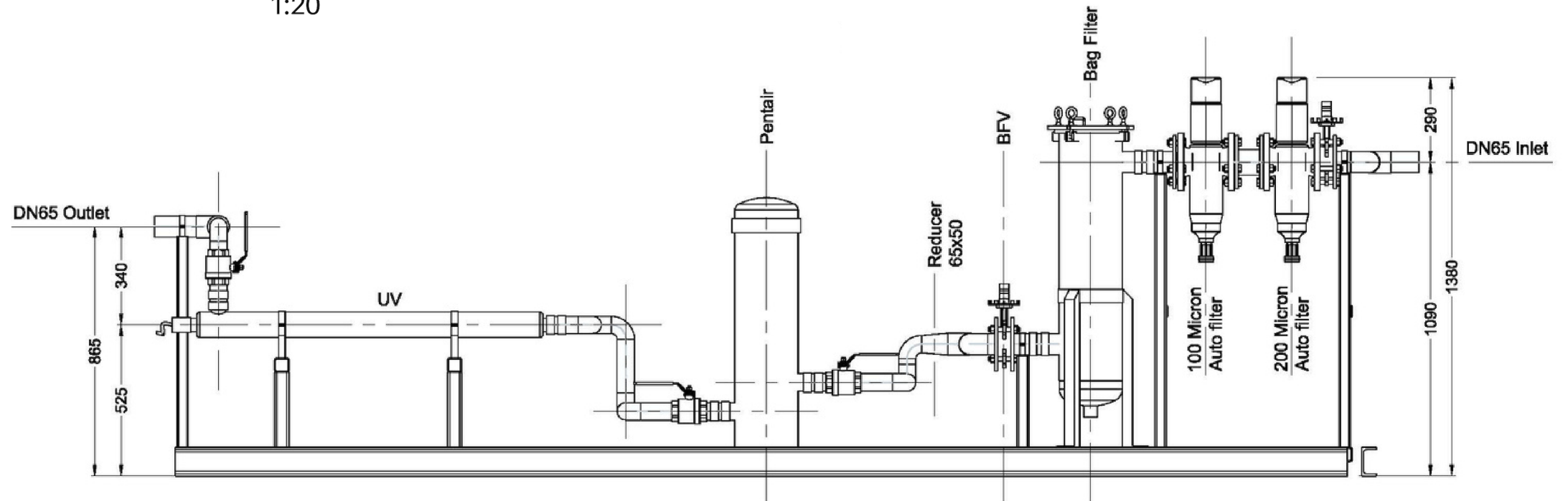
FRONT VIEW
